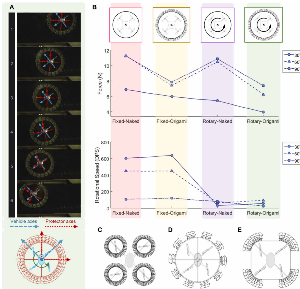
Fig. 6. Analysis of experimental results. (A) Snapshots from high-speed camera videos for an oblique collision with a rough surface at a contact angle of 30° for the origami-protected system in the rotary configuration. Although the protector axes (red) rotate significantly upon impact to the surface, the orientation of the vehicle body axes remains almost invariant. (B) Summary of all results (values averaged between rough and smooth surfaces) demonstrating that the Rotary-Origami (Rotorigami) configuration is the most advantageous design configuration in terms of the overall impact resilience quality. (C to E) A series of conceptual designs for origami-protected aerial robots.
