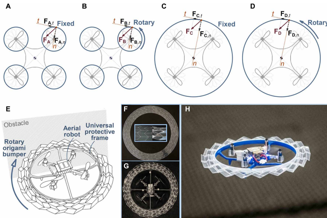
Fig. 1. Conceptual analysis, design, and development of Rorigami for quadcopters. (A to D) Graphical representations of four mechanical protection systems: (A) fixed individual propeller protector, (B) rotary individual propeller protector, (C) fixed universal protector, and (D) rotary universal protector. (E) Rotary universal protector with origami cushion. (F) Laser-cut pattern and its detailed view before and after folding along its perforated crease lines. (G) A miniature quadcopter equipped with Rorigami (Rotary Origami Protective System) in a plan view and (H) in flight.
