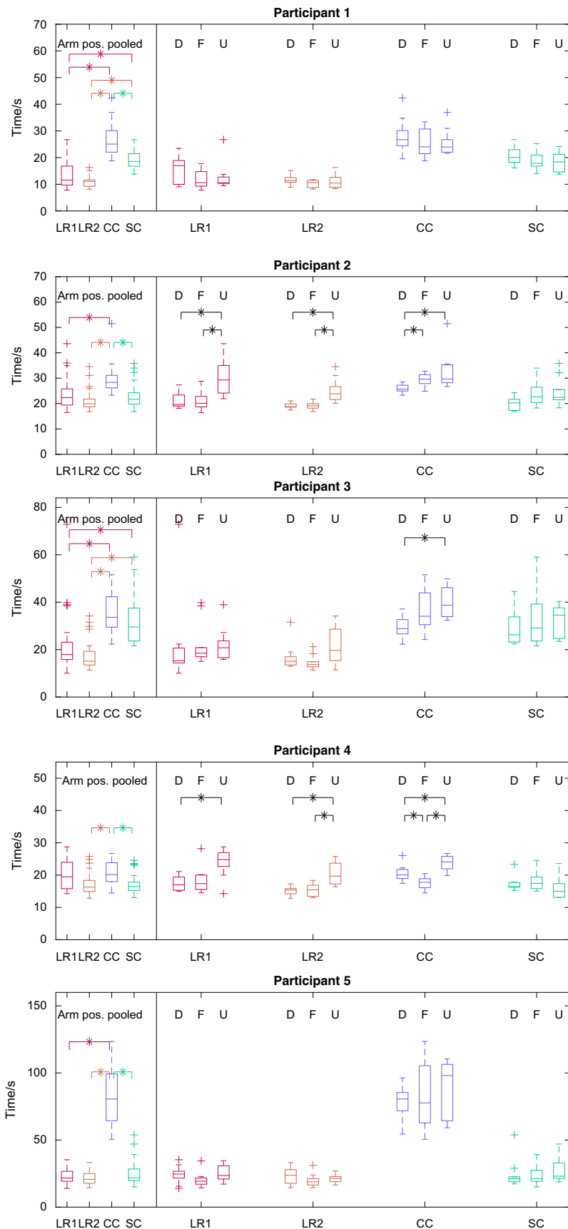
Fig. 1. Results from clothespin relocation test. The time required to transfer three pins from a horizontal to a vertical bar is shown. Performance of LR-based control on two different days without retraining (LR1 and LR2) and two conventional control strategies, CC and SC, is shown separately for each participant (one panel each). The three arm positions—down (D), frontal (F), and up (U)—are shown separately on the right and pooled on the left. The proposed regression-based control outperformed CC for all participants and performed similarly to or better than SC. It was robust against session transfer and less affected by a change of arm position than CC. Asterisks indicate significant differences; plus signs indicate outliers; error bars indicate 25th and 75th percentiles.
