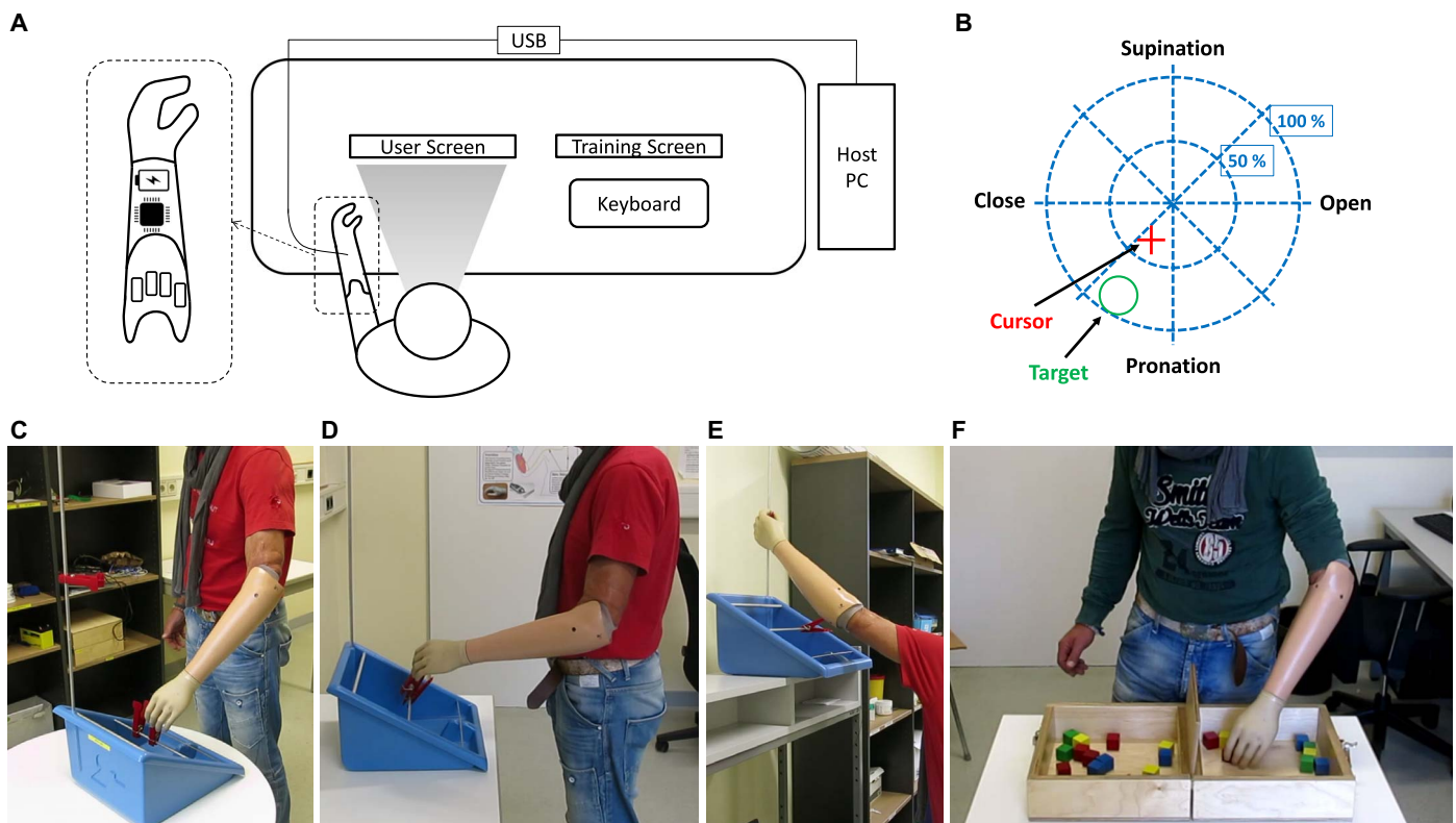
Fig. 3. Experimental setup. (A) Setup for PC-supported user training with regression algorithm. During training, the prosthesis was connected to a PC to record EMG signals while the user received instructions via the user screen. An initial regression model was applied for virtual control tasks for training the user in a game-like software framework and optional co-adaptive learning between the user and the algorithm. (B) Computer game for training the user in conducting noncombined and combined motions of different activation levels with the regression-based control. Evaluation in the clothespin relocation test, executed in arm positions down (C), frontal (D), and up (E). (F) Evaluation in the box-and-blocks test.
