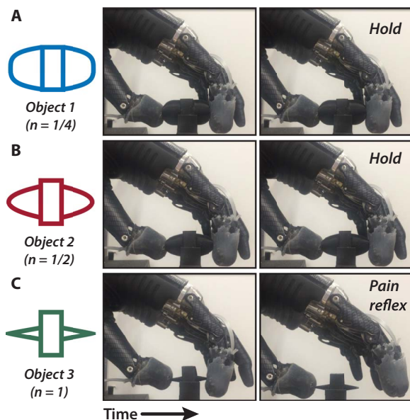
Fig. 5. Prosthesis grasping and control. To demonstrate the ability of the prosthesis to determine safe (innocuous) or unsafe (painful) objects, we performed the PDT. The objects were (A) object 1, (B) object 2, and (C) object 3, each of which is defined by their curvature. In the case of a painful object (object 3), the prosthesis detected the sharp pressure and released its grip through its pain reflex (movie S3).
