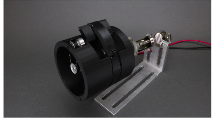
Movie 3. Motorized 4R cylindrical developable mechanism. A possible walking or active-gripping motion is demonstrated.
