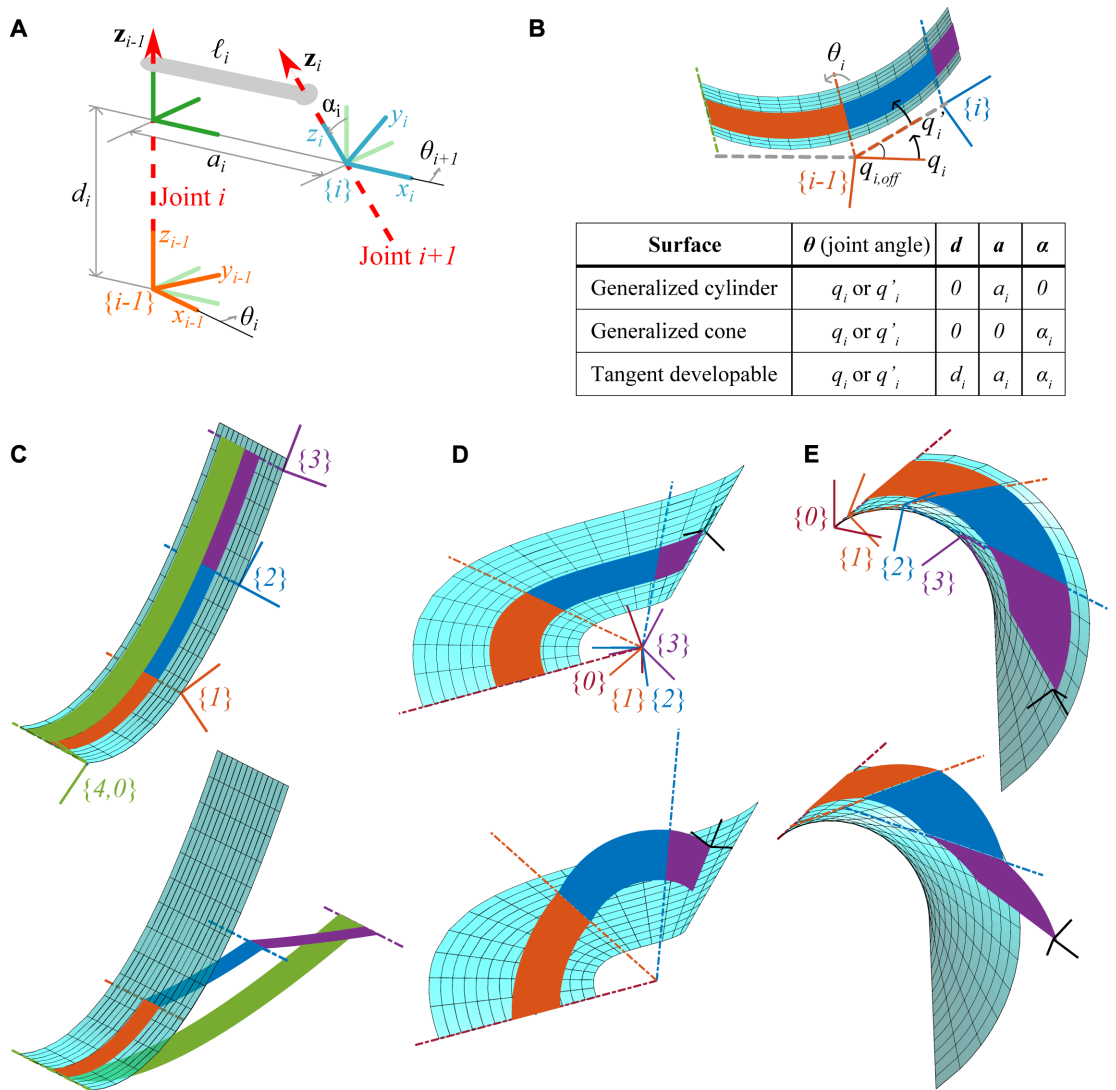
Fig. 6. DH parameters for developable mechanisms. (A) DH parameter notation. (B) Illustration of the introduction of an offset q_{i,off} at the i th revolute joint to change the zero angle reference position from the q_i axis to the q'_i axis, resulting in the zero angle position of the mechanism being the position where the links conform with the surface. The table shows which DH parameters are zero for each type of developable surface. (C) The DH frames on a closed-loop 4R cylindrical developable mechanism in a conforming position (top) and actuated position (bottom). (D) The DH frames on an open 3R chain conical developable mechanism in a conforming position (top) and actuated position (bottom). (E) The DH frames on an open 3R chain tangent developable mechanism in a conforming position (top) and actuated position (bottom). In (D) and (E), a possible tool frame at the end of the chain is shown in black.
