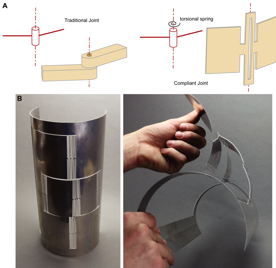
Fig. 4. Compliant joints and developable mechanisms. (A) Compliant flexures can be used in place of traditional hinges to further integrate the linkage into or onto a surface. (B) The stowed and deployed configurations of a compliant cylindrical developable mechanism. Useful mechanisms can be created with 2D manufacturing techniques to be later formed to the desired developable shape.
