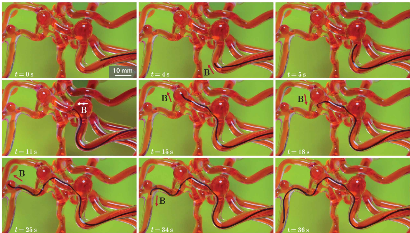
Fig. 6. Demonstration of navigating through a 3D cerebrovascular phantom network. The soft continuum robot first passed through the sharp corner with acute angulation (between t = 0 s and t = 5 s). The robot made another sharp turn after reaching the first aneurysm ( t = 11 s) based on the magnetic steering capability to reach the second aneurysm ( t = 15 s). Then, it made another sharp turn at the acute-angled corner beneath the second aneurysm ( t = 18 s) to reach the third aneurysm ( t = 25 s) and navigated further downstream ( t = 36 s). Magnetic fields for actuation (20 to 80 mT) were generated by a cylindrical (diameter and height of 50 mm) permanent magnet at a distance (40 to 80 mm). The proximal end was pushed to advance the magnetically steered distal end of the robot during the navigation. The outer diameter of the demonstrated prototype was 600 \mu\text{m} . Note that the continuum robot may look thicker than the actual size due to the magnifying effect of the round, thick-walled silicone vessel. Detailed anatomy and dimensions of the phantom model are provided in fig. S7.
