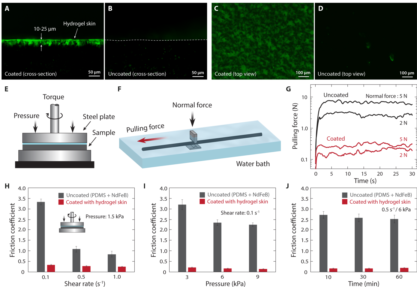
Fig. 2. Hydrogel skin as a lubricating layer. Cross-sectional views of (A) the coated specimen of PDMS + NdFeB (20 volume %) with hydrogel skin visualized by absorbed fluorescein and (B) the uncoated specimen without hydrogel skin. The dashed line in (B) indicates the boundary of the cross-section of the uncoated specimen. Top views of (C) the coated specimen with hydrogel skin and (D) the uncoated specimen. The fluorescing specks visible in the uncoated sample were due to residual fluorescein adsorbed onto the surface. (E) Schematic of testing setup for measuring friction coefficients using a rheometer. (F) Schematic of testing setup for measuring force required to pull a cylindrical specimen (diameter of 8 mm) at a constant speed under applied normal force by the pair of grips. (G) Semi-log plot of the pulling force measured over time during the pullout test performed at 200 \text{ mm min}^{-1} for both coated and uncoated specimens under two different normal force conditions (2 and 5 N). Friction coefficients measured from both coated and uncoated samples under different (H) shear rates and (I) normal pressure. (J) Friction coefficients measured from prolonged shearing of both coated and uncoated samples up to 60 min at shear rate of 0.5 \text{ s}^{-1} under normal pressure of 6 kPa. The error bars in (H) to (J) indicate the SDs of the mean values obtained from five different measurements.
