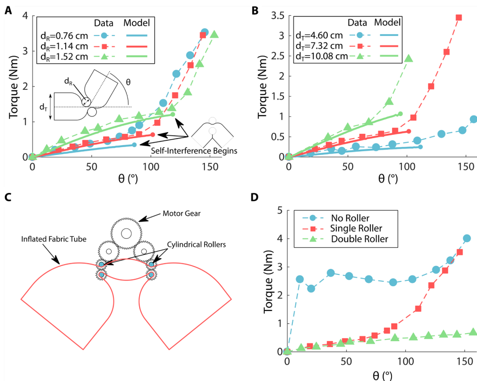
Fig. 6. Analysis of the effective joint formed by rollers pinching a tube. (A) The relationship between angle and torque with changing roller diameter (tube diameter is 7.32 cm). Model predictions are shown in solid lines, and experimental data are shown in dashed lines. The model slightly underpredicts the torque. The amount of torque increases substantially beyond the point where the model predicts self-interference. Torque increases with roller size, but interference also begins at larger angles. (B) Increasing torque with increasing tube diameters when the roller diameter is 1.14 cm. (C) Double roller configuration and the gear train that ensures all rollers move together from a single motor input. (D) Torque required to bend a tube with no rollers, with a single set of rollers, and with two sets of rollers as shown in (C) (roller diameters are 0.64 cm separated by 6.35 cm). Without rollers, the tube exhibits low stiffness, but large torque at a wide range of angles. The presence of one set of rollers markedly reduces the torque at low angles, but the torque rises quickly after self-interference begins. With two sets of rollers, the torque is low for small and large angles because the tube does not self-interfere.
