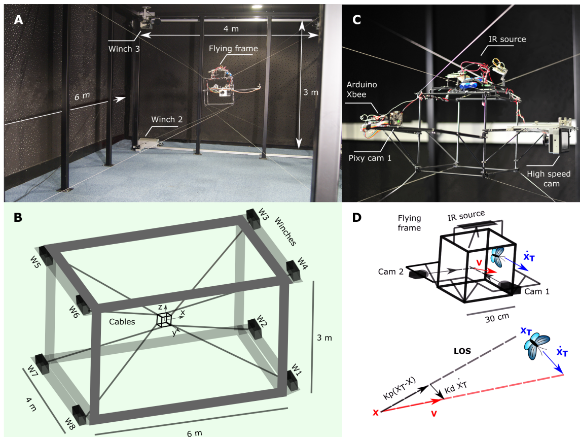
Fig. 2. Lab-on-cables setup. (A) Photo of the cable robot (6 m by 4 m by 3 m) and (B) schematic view of the setup. (C) Photo of the flying frame (30 cm by 30 cm by 30 cm). The flying frame supports the lab equipment, i.e., an IR source and a pair of calibrated cameras (Pixy cam 1 and 2), for online insect location. The flying frame moves automatically to keep the insect within the detection range of the cameras. (D) Robot control as deviated pursuit. Robot and insect locations are X and X_T , respectively. The insect speed is denoted \dot{X}_T . The tracking speed V is the sum of a pure pursuit term pointing along the line of sight (LOS) toward the target current location and a corrective term, taking into account the direction of motion of the target. This is like anticipating where the target will be to point ahead of the target and cover less distance.
