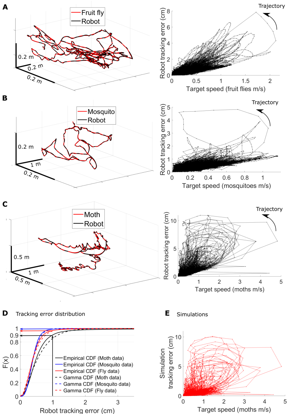
Fig. 3. Tracking prerecorded insect trajectories. (A to C) Left: Examples of insect trajectories (red curves) versus robot trajectories (black curves). Right: Tracking errors of the robot (in centimeters) versus flight speed of the insect (in meters per second). (D) Cumulative distributions of the tracking error for experimental data (plain curves) and theoretical gamma distribution (dashed curves). (E) Tracking errors of the simulated model (Euler integration of Eq. 1) versus flight speed of the insect (moth data).
