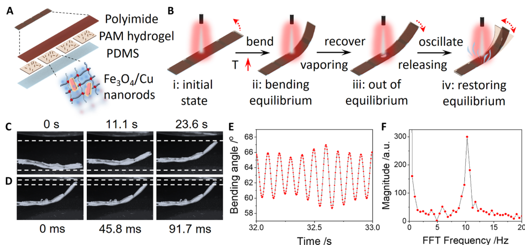
Fig. 1. Photothermal oscillators powered by local steam generation. (A) Schematic illustration of the trilayer structure of the actuators. (B) Working mechanism of the hydrogel oscillation driven by photothermal steam generation. Digital photos showing the (C) bending and (D) oscillation of the actuators under NIR light irradiation. (E) Time-resolved bending angles during oscillation. (F) Corresponding FFT of the bending angles. a.u., arbitrary units.
