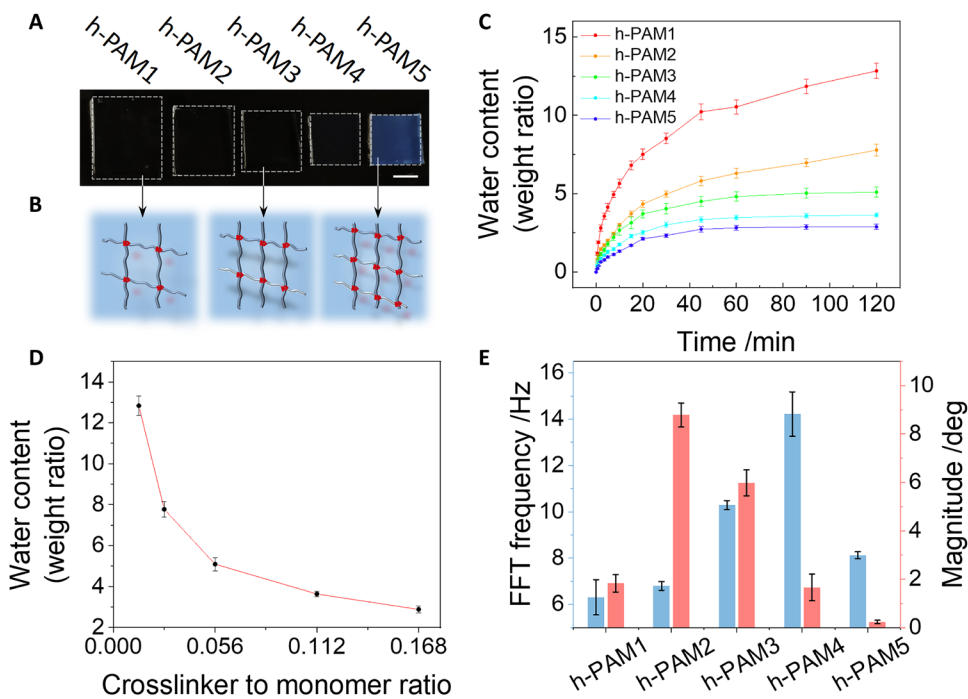
Fig. 3. Tuning oscillation frequency by controlling the hydrogel cross-linking ratio. (A) Digital pictures and (B) schemes of the hydrogel films with different cross-linking ratios. Scale bar in (A): 0.5 cm. (C) Hydration performance of the hydrogel films with different cross-linking ratios. (D) Dependence of water content on hydrogel cross-linking ratios. (E) Dependence of oscillation frequency and magnitude of the hydrogel oscillators on cross-linking ratios. Error bars indicate SD based on three measurements.
