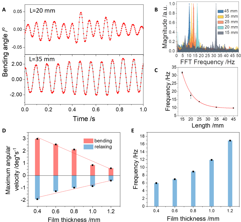
Fig. 2. Tuning the oscillation frequency by controlling film geometry. (A) Oscillation amplitude of films with different lengths. (B) FFT of film oscillation for different lengths. (C) Dependence of oscillation frequency on film length. Error bars indicate SD based on three measurements. (D) Dependence of maximum bending and relaxing velocity of the trilayer oscillators on the film thickness. (E) Oscillation frequency as a function of film thickness. a.u., arbitrary units.
