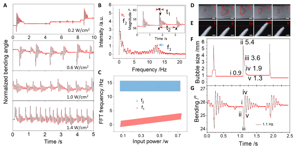
Fig. 4. Pulsed and damped harmonic photothermal oscillation. (A) Hydrogel oscillation under NIR light irradiation with different input energy. (B) FFT of the hydrogel oscillation. Inset defines the oscillation periodicity ( t_1 ) and pulse periodicity ( t_2 ). (C) Dependence of the oscillation ( f_1 ) and pulse frequency ( f_2 ) on light intensity. (D) Digital pictures of the steam bubble evolution and (E) the coherent film bending under NIR light irradiation. Scale bars in (D) and (E): 2 mm. (F) Time-resolved steam bubble size and (G) film bending angles. (i), (ii), (iii), (iv), and (v) in (D) to (G) represent the initial equilibrium state, state with maximum bubble size, and states under the first, second, and third oscillation peaks of the middle pulse in (G), respectively. The values in (F) represent corresponding bubble diameters in millimeters in the five states. a.u., arbitrary units.
