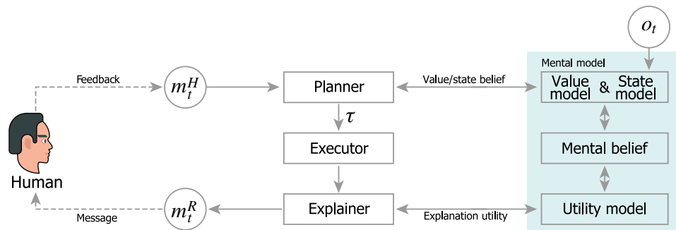
Fig. 6. Algorithmic flow of the computational model. Given game observations and human feedback to previous proposals, the robots update their mental state and make new task plans. On the basis of the plans and current beliefs, new proposals and explanations are generated and sent to the human for feedback in the next round.
