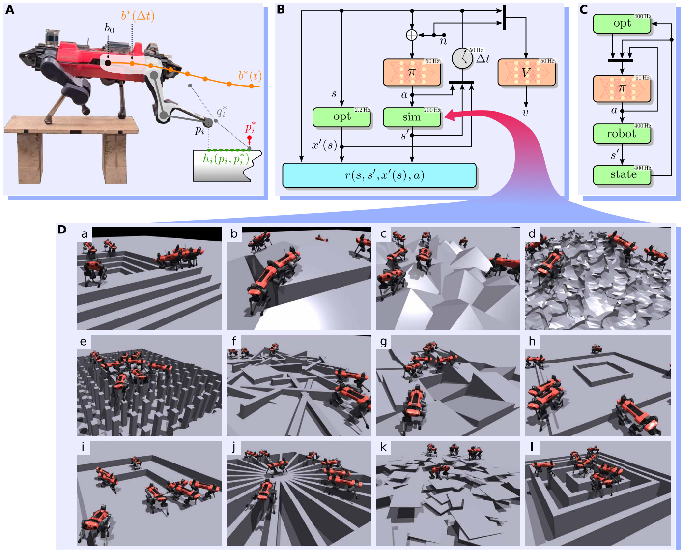
Fig. 8. Overview of the training method and deployment strategy. (A) The optimized solution provides footholds p_i^* , desired base pose b^* , twist b^* , and acceleration \ddot{b}^* (extracted one policy step \Delta t ahead), as well as desired joint positions q^* . In addition, a height scan h is sampled between the foot position p_i and the corresponding foothold. (B) Training environment: The optimizer runs in parallel to the simulation. At each leg touchdown, a new solution x' is generated. The policy \pi drives the system response s' toward the optimized solution x'(s) , which is encouraged using the reward function r . Actor observations are perturbed with the noise vector n , whereas critics and the TO receive ground truth data. (C) Deployment: Given the optimized footholds, the network computes target joint positions that are tracked using a PD control law. The state estimator (state) returns the estimated robot state, which is fed back into the policy and the optimizer. (D) The list of terrain types includes (a) stairs, (b) combinations of slopes and gaps, (c) pyramids, (d) sloped rough terrain, (e) stepping stones, (f) objects with randomized poses, (g) boxes with tilted surfaces, (h) rings, (i) pits, (j) beams, (k) hovering objects with randomized poses, and (l) pallets.
