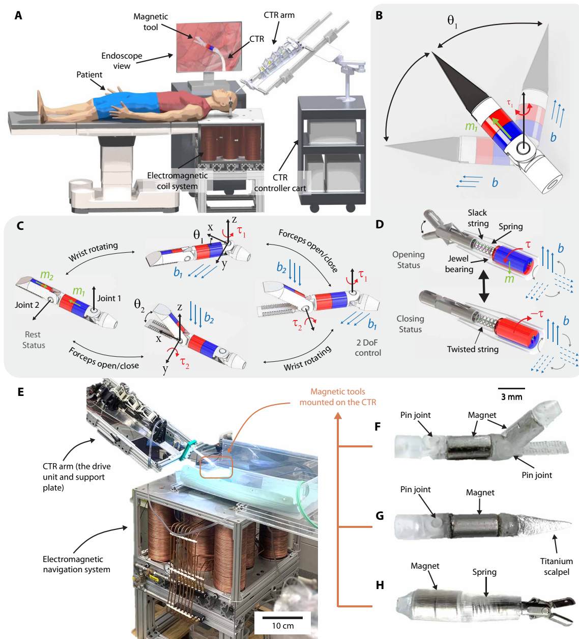
Fig. 2. The proposed magnetic robotic system. (A) Overview of the system that includes magnetic tools, an electromagnetic navigation system, a CTR arm, and an endoscopy system. (B) Illustration of the magnetic pivoting scissors design. (C) Illustration of the magnetic wristed gripper design. (D) Illustration of the magnetic TSA forceps design. (E) The developed multicomponent magnetic robotic system and images of fabricated magnetic tools, namely, (F) the wristed gripper, (G) the pivoting scalpel, and (H) the TSA forceps.
