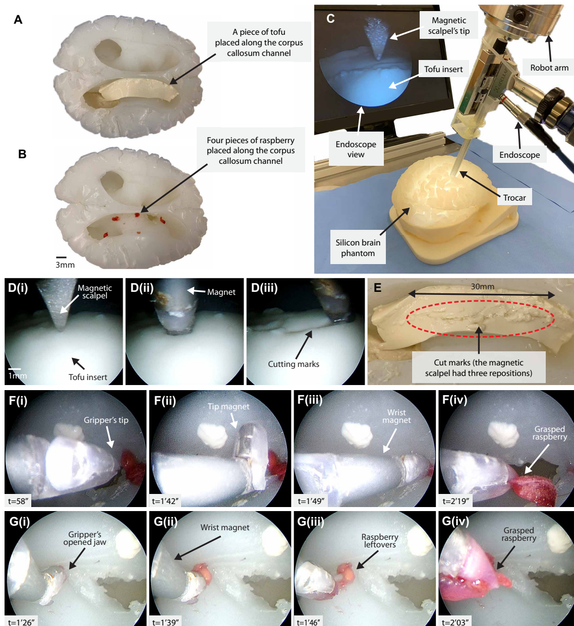
Fig. 3. Magnetic robots operate on the brain phantom. (A) A piece of tofu was placed in the brain phantom to mimic the corpus callosum. (B) Four small pieces of raspberry were placed along the corpus callosum area to mimic the tumor tissue. (C) The magnetic tool was positioned by a robot arm and inserted into the brain through the trocar's working channel with endoscopic visual feedback. (D) (i to iii). The magnetic scalpel inserted into and cut the tofu by pivoting its blade. (E) The tofu cut trace made by the magnetic scalpel. The magnetic wristed gripper picked up a piece of raspberry that was placed in the phantom's (F) (i to iv) right side and (G) (i to iv) left side.
