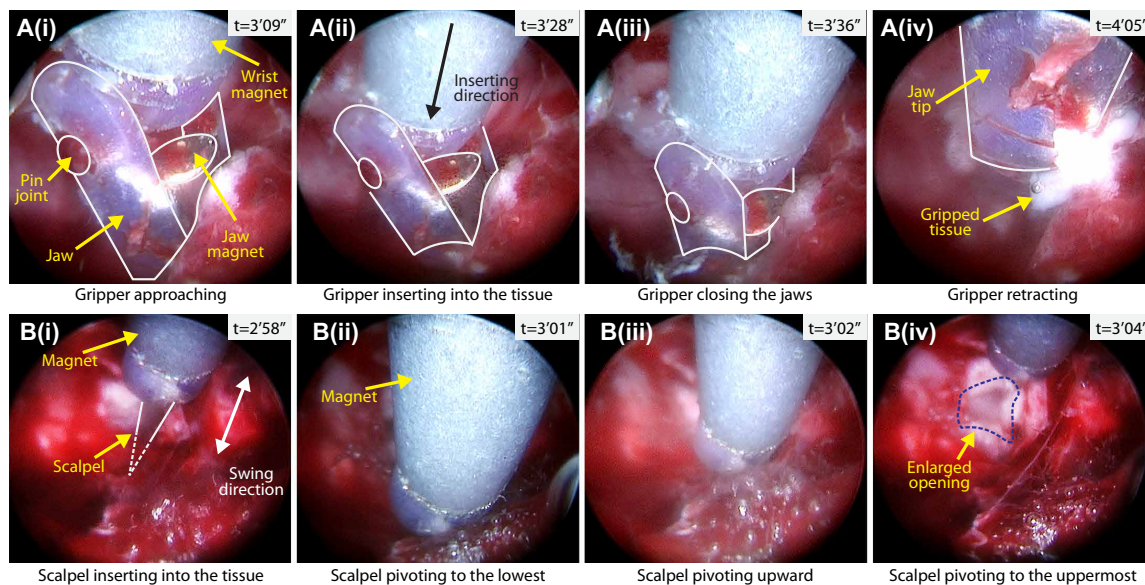
Fig. 6. Magnetic robots operate in the ventricle of the piglet brain. (A) (i to iv): The magnetic gripper was controlled to grip the tissue around the ventricle after its wrist was adjusted to the desired direction. (B) (i to iv): The magnetic scalpel was controlled to cut the tissue, creating an incision to access the ventricle.
