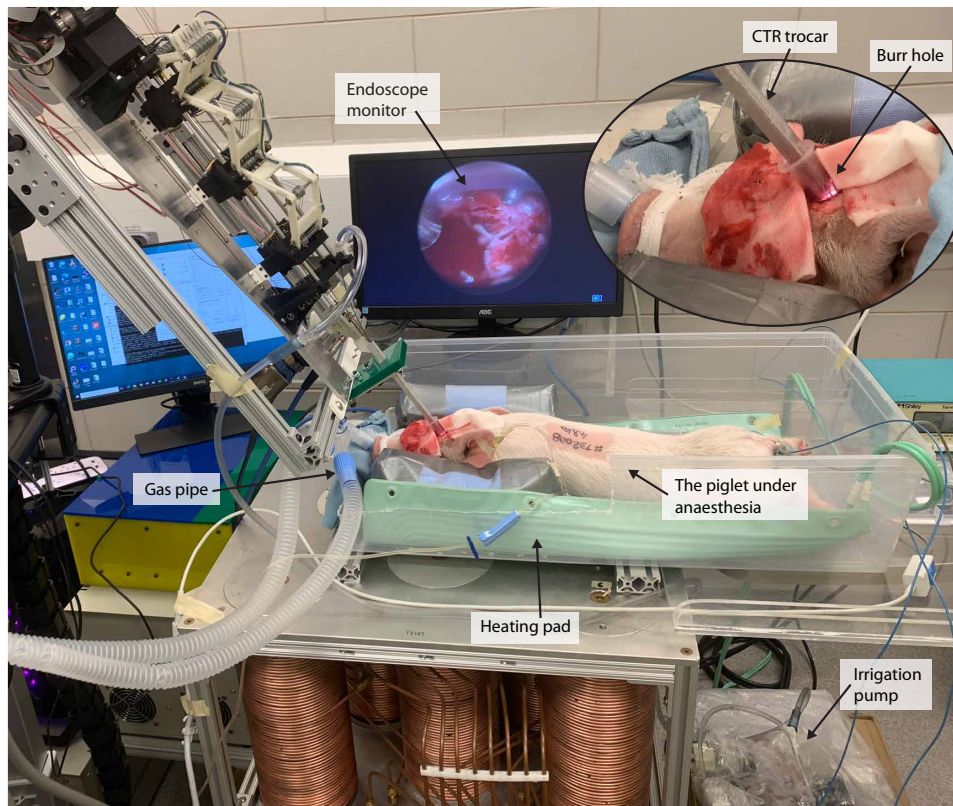
Fig. 4. The operating room setup for the in vivo experiment. The anesthetized piglet was placed with its head right above the ENS system table center. A burr hole was created on the piglet's skull that provided the entry to insert the trocar into the brain.
