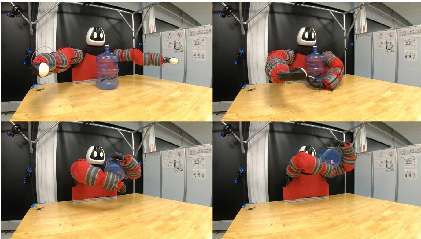
Movie 3. Hardware rollout of the blind (no object pose tracking, only proprioceptive-and-tactile feedback), jug-over-shoulder policy.
