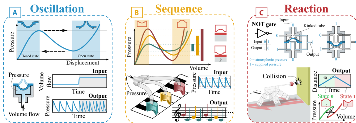
Fig. 1. Self-regulating oscillation, sequence, and reaction as fundamental features of physical control. (A) Oscillation. In a fluidic relaxation oscillator, a single steady input is converted into a periodic oscillation, harnessing the unique characteristics of a snap-through membrane with slits (2). The membrane snaps between two states when the pressure exceeds a peak or valley threshold. In one state, the slits remain closed (pressure builds up, no volume flow), and in the other, they open (pressure is released, allowing high-volume flow). When the membrane is loaded by a constant volume flow, a spontaneous oscillation emerges, with a frequency that is linked to the magnitude of the volume flow. (B) Sequence. A single modulated input generates a discrete sequence of multiple outputs, harnessing the snapping characteristics of conical shells. By interconnecting multiple fluidic snapping actuators, with different snapping pressures, to the same pressure input, a robotic system can play a melody on a piano by simply modulating the input pressure between snapping thresholds (4). (C) Reaction. Boolean logic is implemented in soft robots using soft bistable valves and realized using snapping membranes that kink tubes to block volume flow (3), functioning as NOT gates. The integration of bistable sensing elements in Boolean fluidic circuits makes soft robots responsive to their environment, switching trajectories when colliding with a wall (7).
